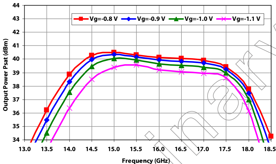
XP1070-BD, Vd=7.5 V, Vg=Varied Pulsed Duty Cycle 1% with 1ms Period
