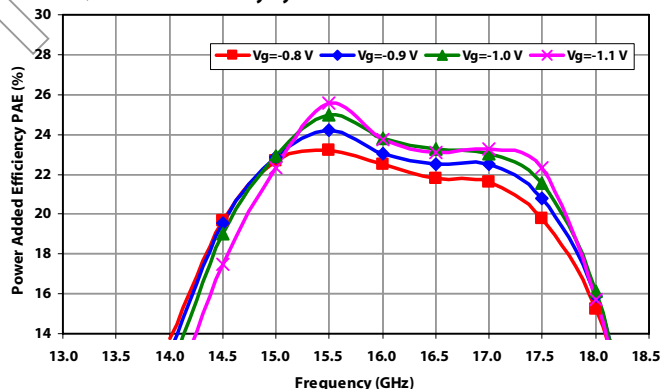
XP1070-BD, Vd=7.5 V, Vg=Varied Pulsed Duty Cycle 1% with 1ms Period
